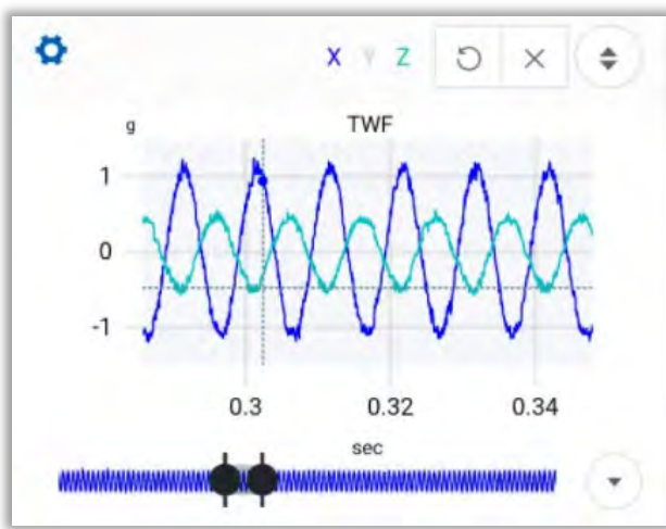
Example TWF and FFT with X & Z axes:
